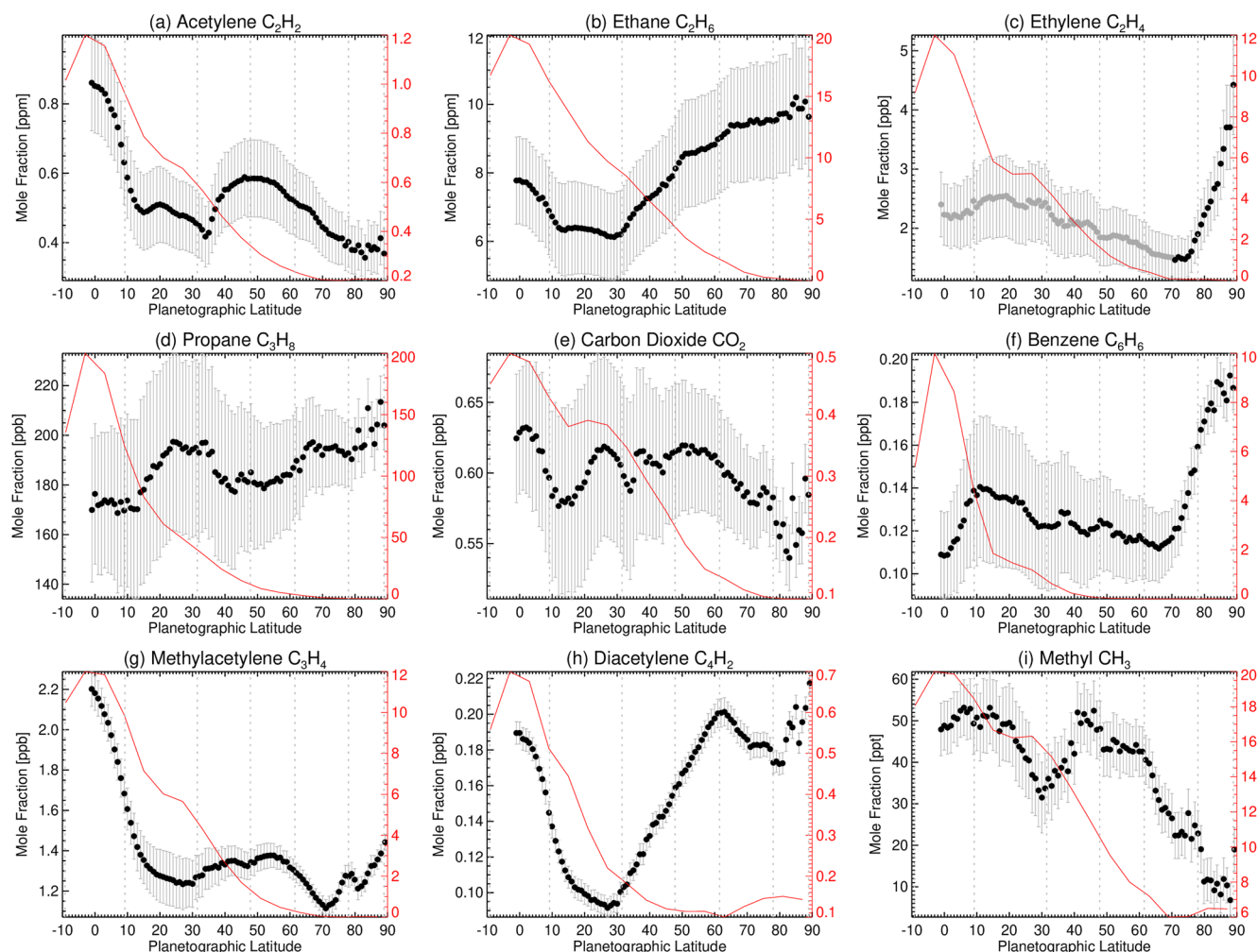
Figure 17. Distributions of stratospheric species at 0.5 mbar: acetylene, ethane, ethylene, propane, \text{CO}_2 , benzene, methylacetylene (propyne), diacetylene (1,3-butadiyne), and methyl in Saturn's northern summer, compared to the predictions of the neutral photochemistry model for L_s = 150^\circ (Moses & Greathouse, 2005; Moses et al., 2007). The photochemical model is shown in red, and is referenced to the right-hand axis so that both the shape of the distribution and differences in absolute abundances can be compared. Error bars are shown in gray, but these do not include uncertainties due to scaling a latitudinally uniform a priori profile. If the shape of the profile changes significantly with latitude (as is expected for benzene and \text{C}_4\text{H}_2 from previous studies), this could influence the retrieved values. Vertical dotted lines show the latitudes of tropospheric eastward jets. Gases in panels (a–c) were derived as full vertical profiles, other gases are derived as scale factors for our a priori profiles. Gray points in panel (c) signify a lack of obvious detection of \text{C}_2\text{H}_4 emission by eye.
