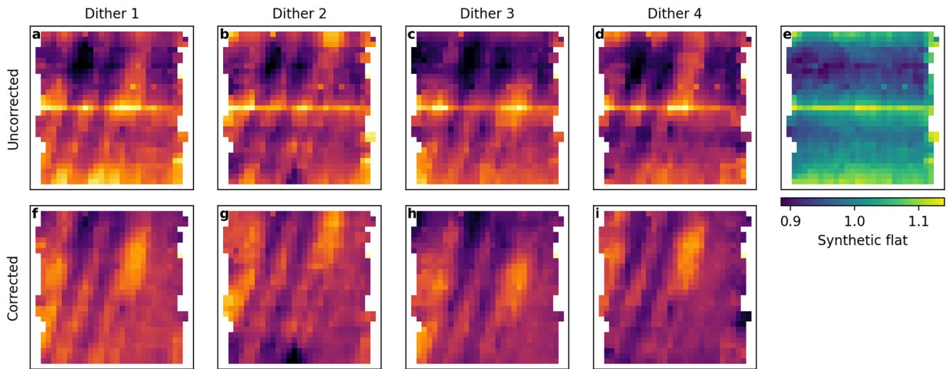
Figure 5. Example images at 5.07\ \mu\text{m} (channel 1-SHORT) before (a–d) and after (f–i) the synthetic flat field field (e) is applied. The images are shown in the integral field unit (IFU) frame, where north is to the top left. The flat field effects in panel (a–e) (such as the bright line across the center of each image) are fixed in the IFU frame, whereas the observed spatial structure on Saturn varies in position on the detector with the different dithers, allowing flat field structure and real spatial structure to be differentiated.
