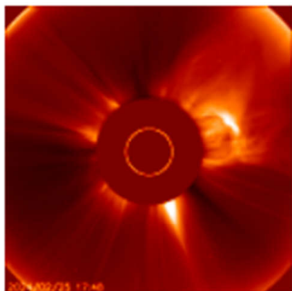
LASCO C2
