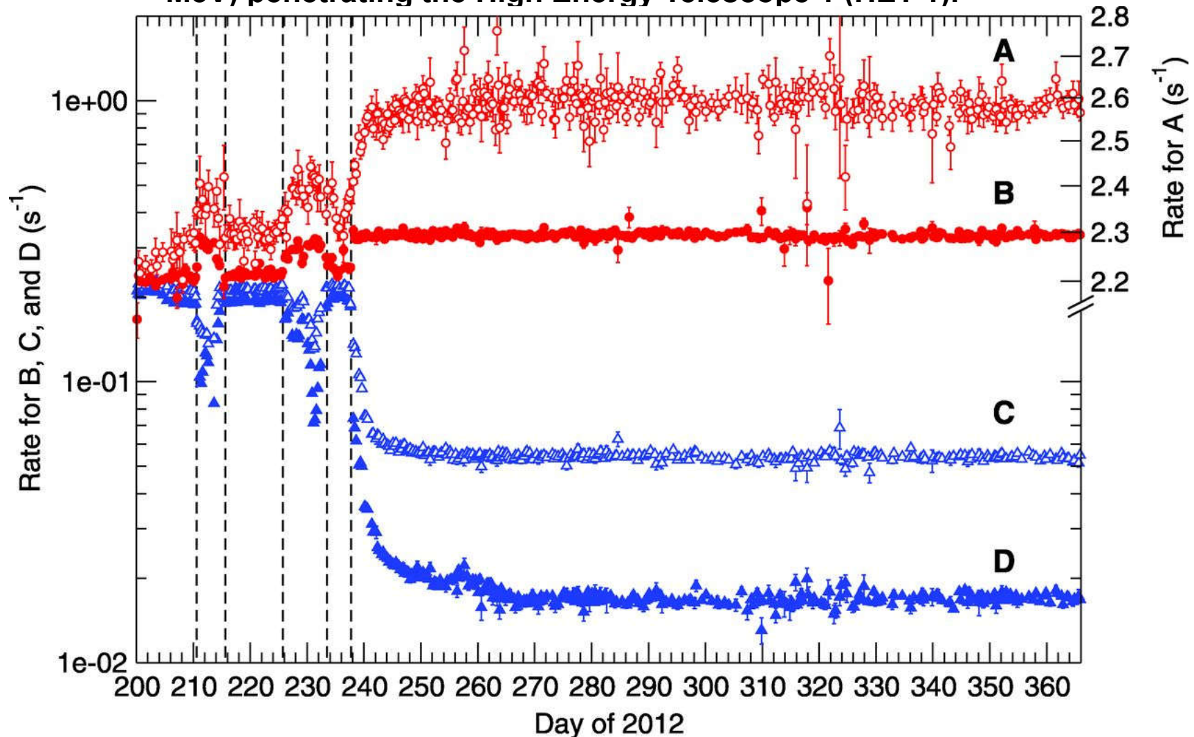
Fig. 1 The counting rates (6-hour averages) of four different energetic particle species in the vicinity of the depletion region.(A) (y axis on right) GCR nuclei (mainly protons with E > 70 MeV) penetrating the High Energy Telescope 1 (HET 1).
