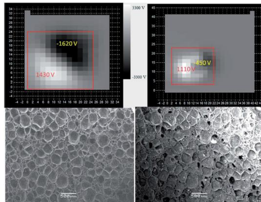
Fig. 2 (Top) Electrostatic potential maps of PTFE film (left) sheared with LDPE foam slabs (right). The electrostatic potential of the positive and negative regions of each material is printed sheared LDPE
