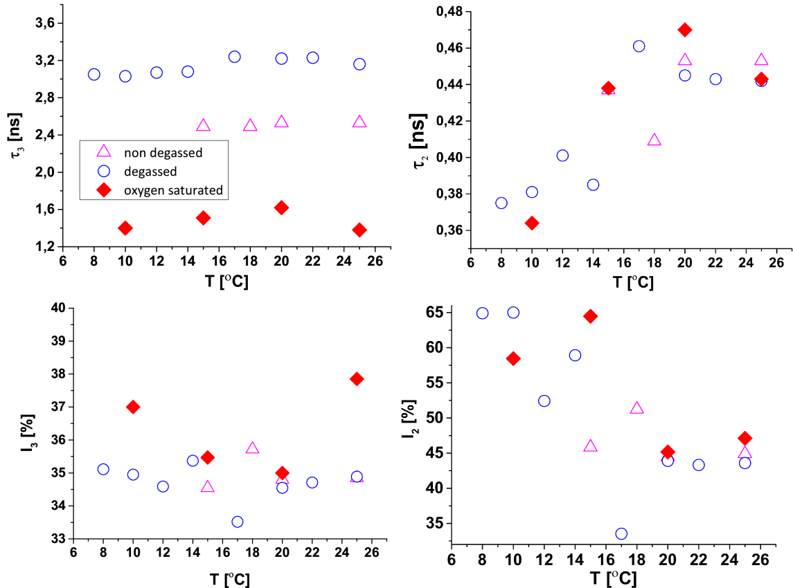
Fig. 1. Positron lifetimes \tau_3 , \tau_2 and intensities I_3 , I_2 as a function of temperature in non-degassed ( \Delta ), degassed ( \circ ) and oxygen-saturated ( \diamond ) cyclohexane ( C_6H_{12} ).
