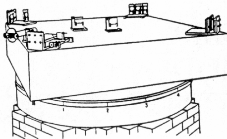
Figure 6 The scheme of Michelson-Morley's apparatus.
