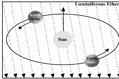
Figure 4 The concept of the aether [8].
