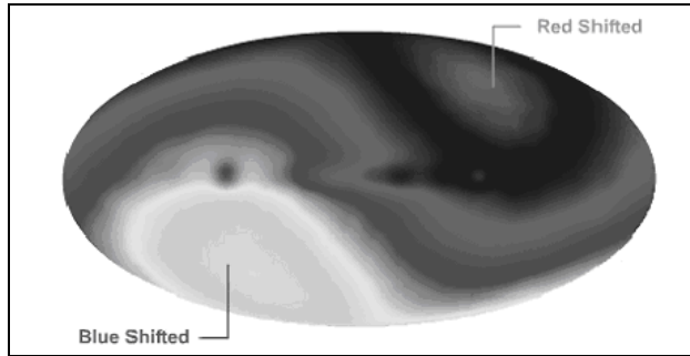
Figure 8 The changes of the temperature ( \pm 3 mK) of the Cosmic Microwave Background measured by COBE. http://csep10.phys.utk.edu/astr162/lect/cosmology/cbr.html
