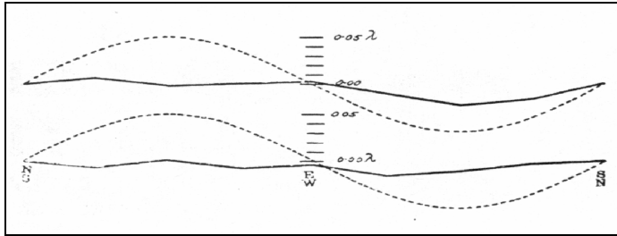
Figure 7 The results of the observations of Michelson and Morley from the paper „On the relative motion of the Earth and the luminiferous aether” [2]. The upper is the curve of observations at noon, and the lower for the evening observations. The dotted curves represent the theoretical displacements.
