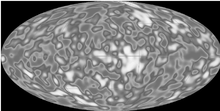
Figure 9 The changes of the temperature ( \pm 27 \mu K) of the Microwave Background Radiation measured by COBE, http://map.gsfc.nasa.gov/m_mm.html .
