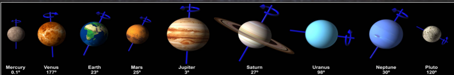
Obliquity of the Nine Planets
