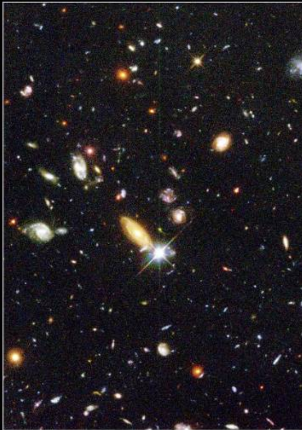
Hubble Deep Field Hubble Space Telescope • WFPC2
