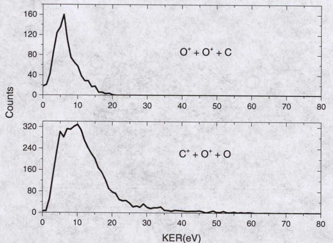
FIG. 2. KER distributions for three-body fragmentation of CO 2 2+ induced by 200 eV electron impact.
