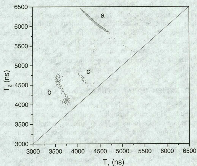
FIG. 1. (Color online) Ion-ion coincidence map obtained in 200 eV electron collision with \text{CO}_2 (raw data). Three pronounced channels are from a , \text{O}^+ + \text{CO}^+ ; b , \text{C}^+ + \text{O}^+ + \text{O} ; and c , \text{O}^+ + \text{O}^+ + \text{C} .
