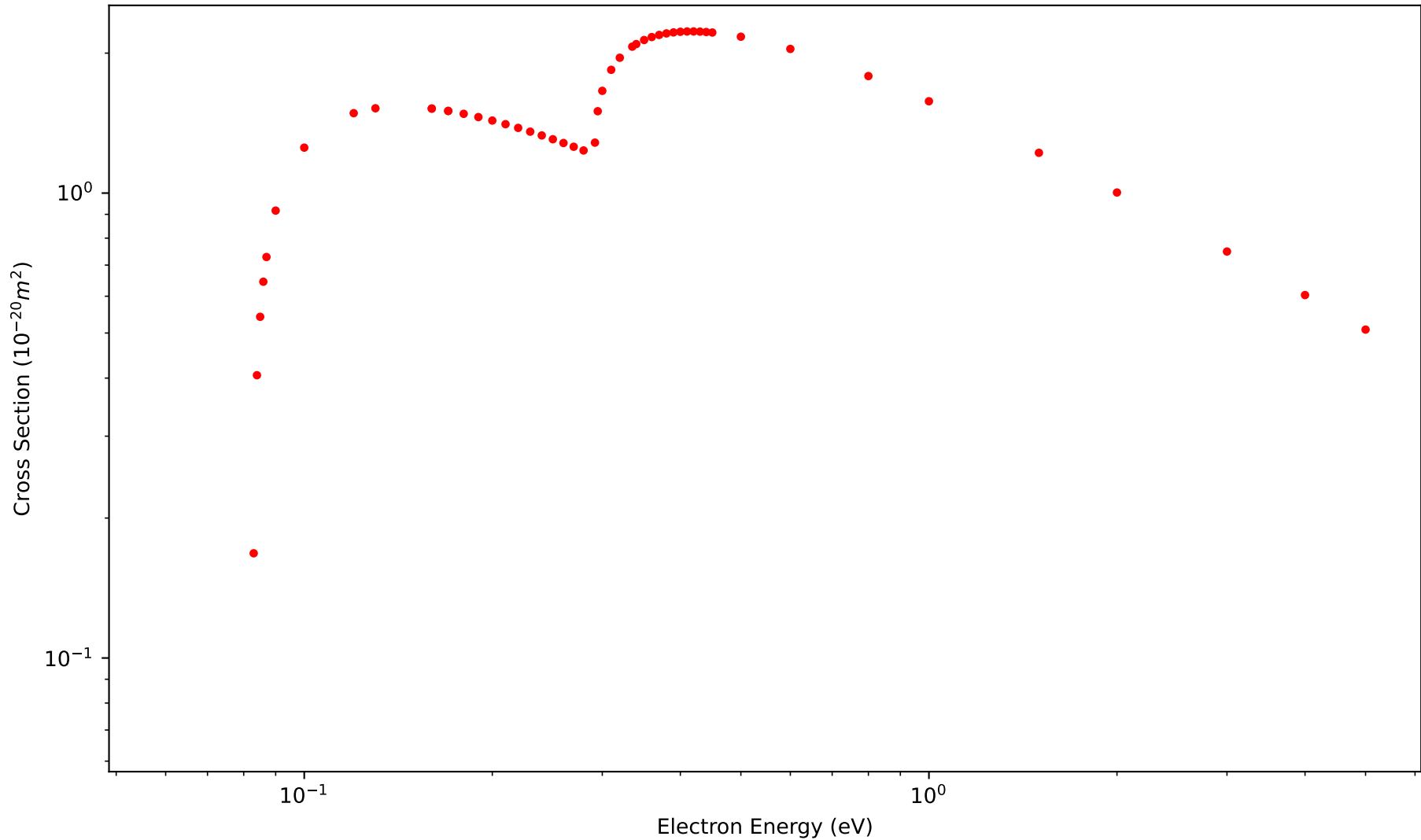
Cross Section vs. Energy for Different Studies
