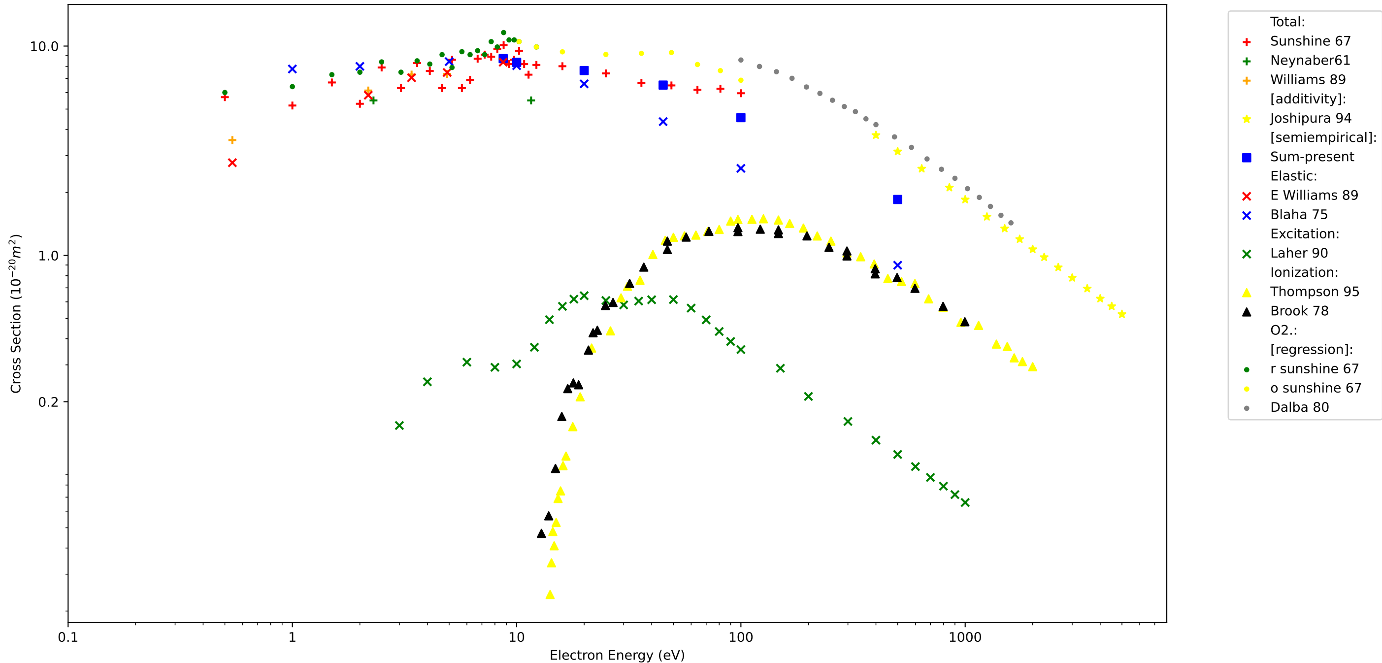
Cross Section vs. Energy for Different Studies
