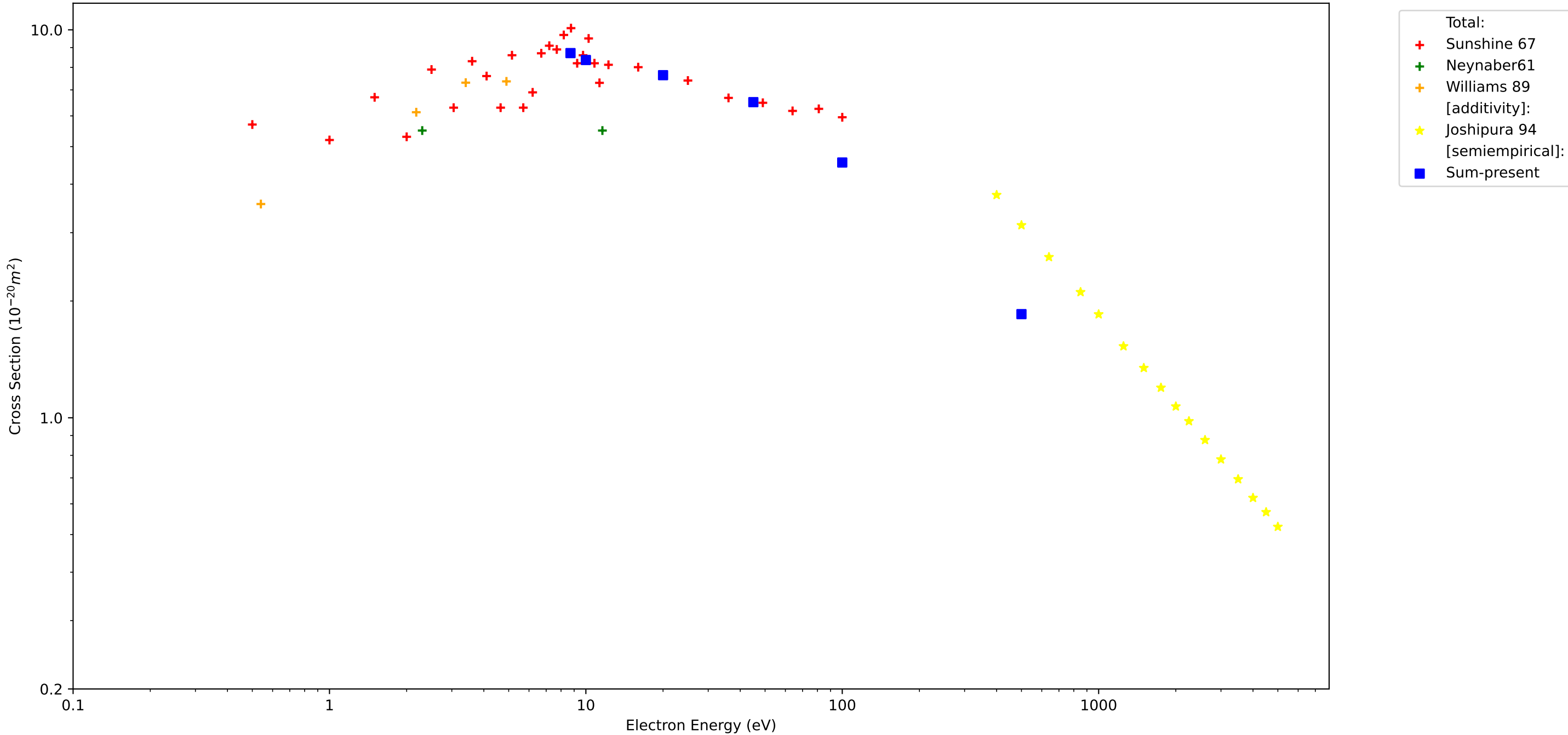
Cross Section vs. Energy for Different Studies
