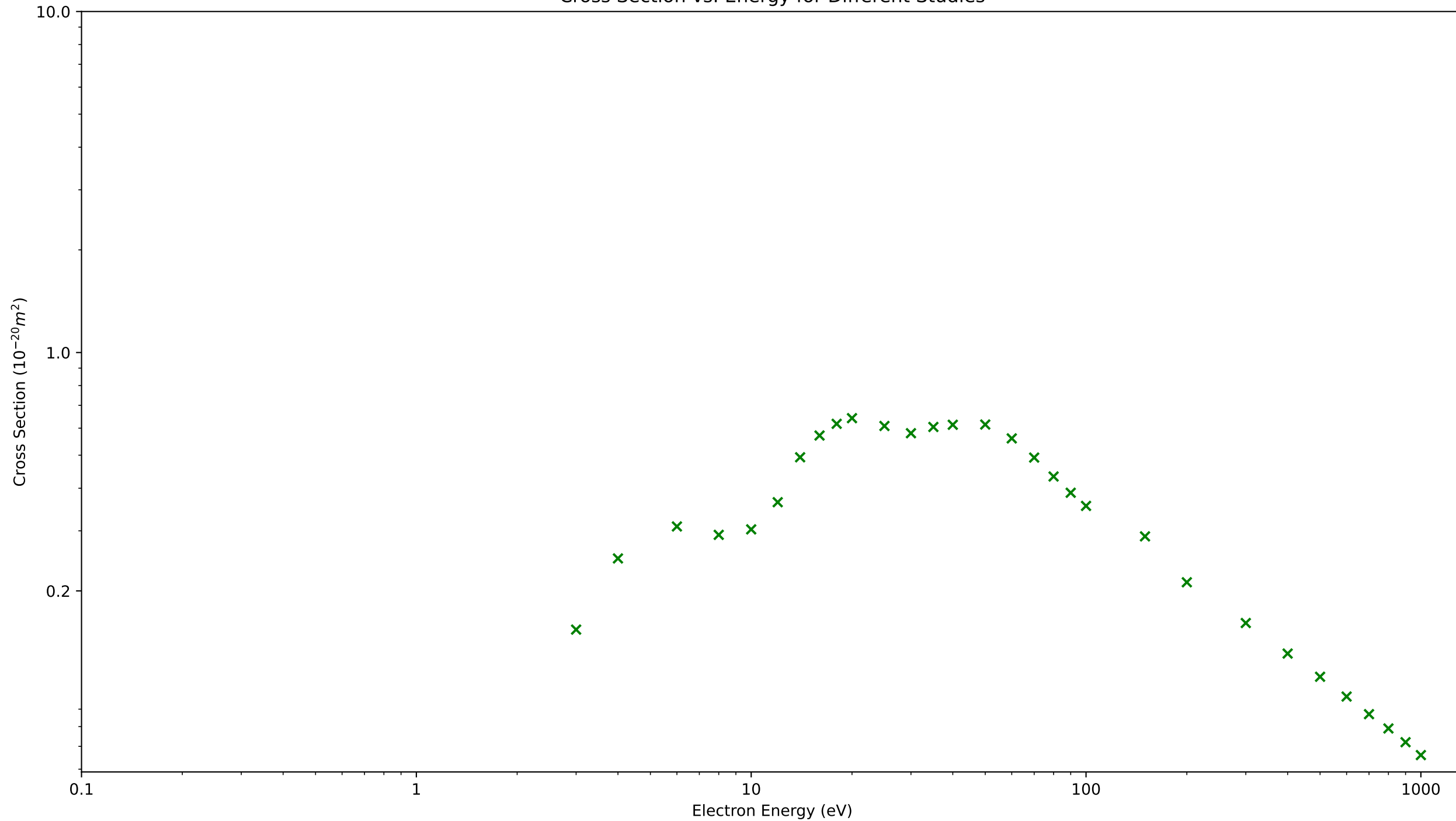
Cross Section vs. Energy for Different Studies
